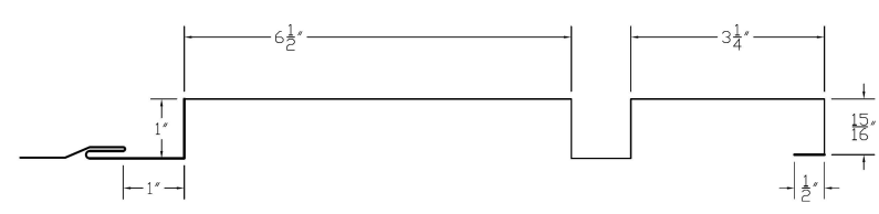
VariPanel™ 63.1 PLANK (SIDEVIEW)
