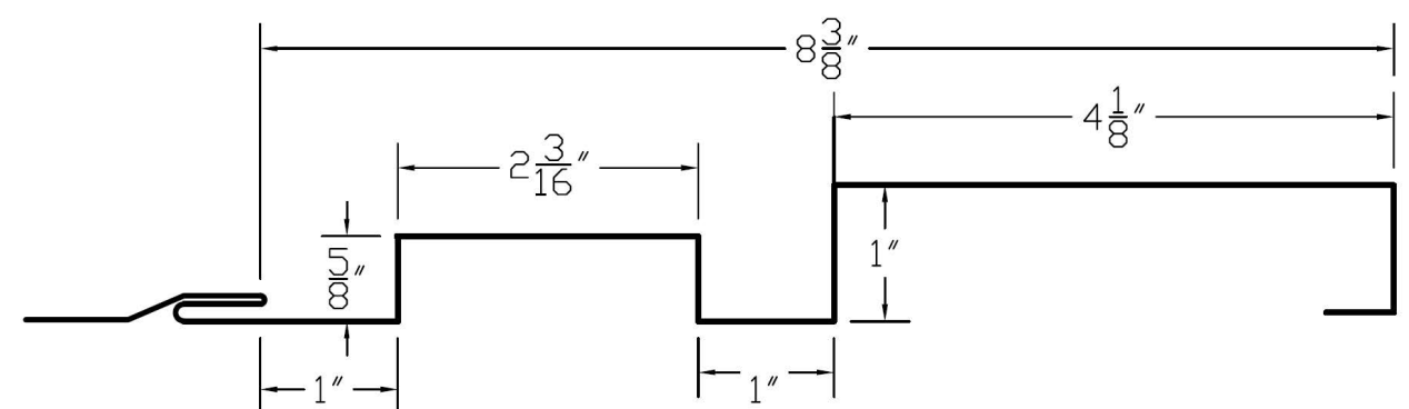
DV 1 PROFILE
