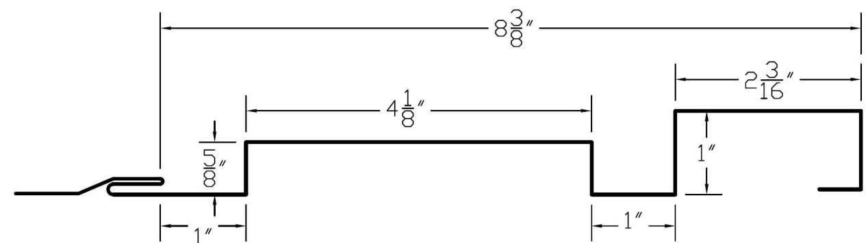
DV 2 PROFILE
