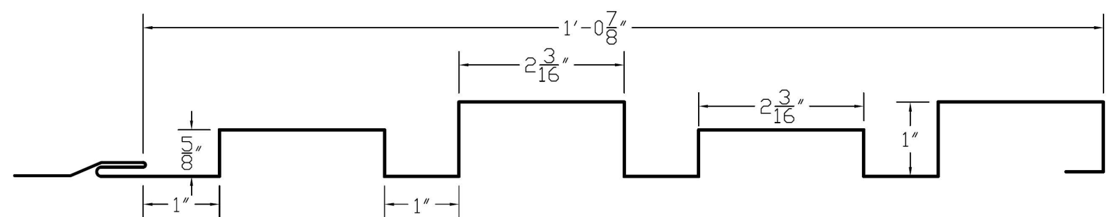
DV 3 PROFILE
