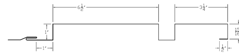
VariPanel™ 63.1 PLANK (SIDEVIEW)
