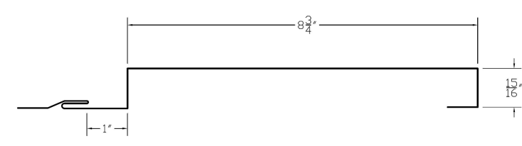
VariPanel™ 9.1 PLANK (SIDEVIEW)
