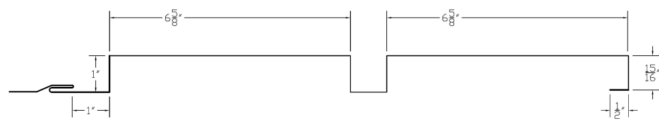
VariPanel™ 77.1 PLANK (SIDEVIEW)
