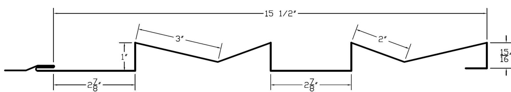
VariPanel™ Angular CONCAVE (SIDEVIEW)
