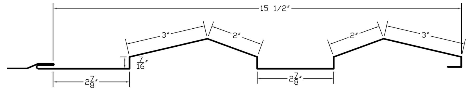
VariPanel™ Angular CONVEX (SIDEVIEW)
