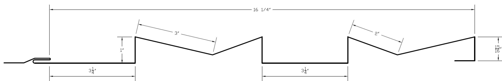
VariPanel™ Angular CONCAVE (SIDEVIEW)
