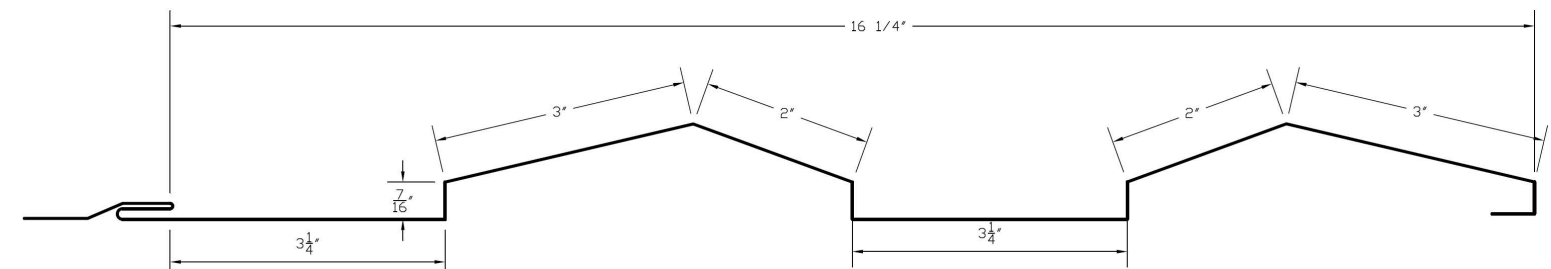
VariPanel™ Angular CONVEX (SIDEVIEW)
